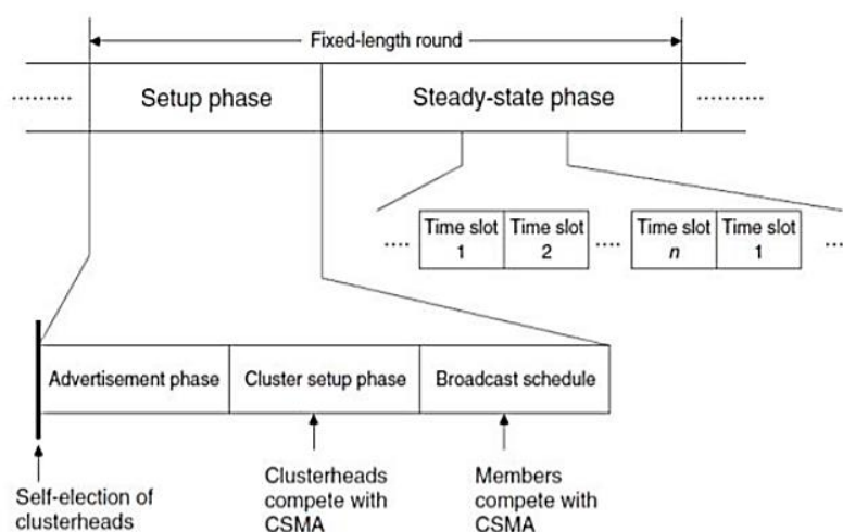
Fig. 1. Timeline operation of leach.
